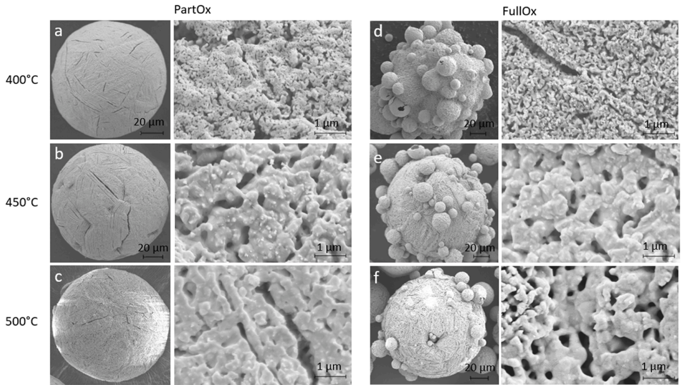
Fig. 8. Scanning electron microscopy (SEM) images with secondary electrons contrast of the surface porosity formed after full reduction of (a-c) PartOx powder and (d-f) FullOx powder at (a, d) 400 °C, (b, e) 450 °C and (c, f) 500 °C in the thermogravimetry (TG) reactor.
